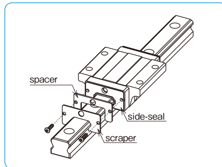
Figure A-26 Scraper
