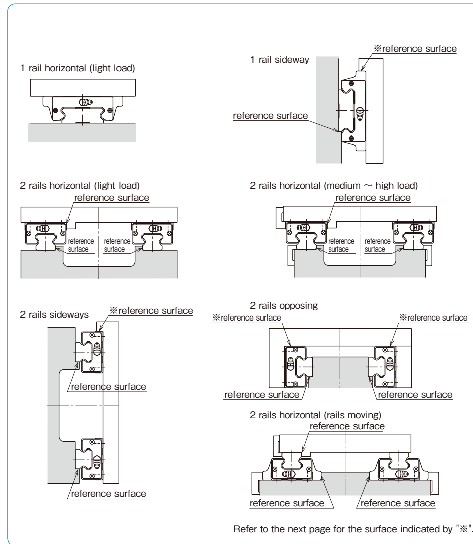
Figure A-6 Slide Guide Arrangements
