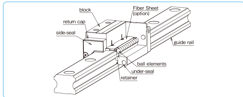
Figure A-54 Structure of SGL type Slide Guide
