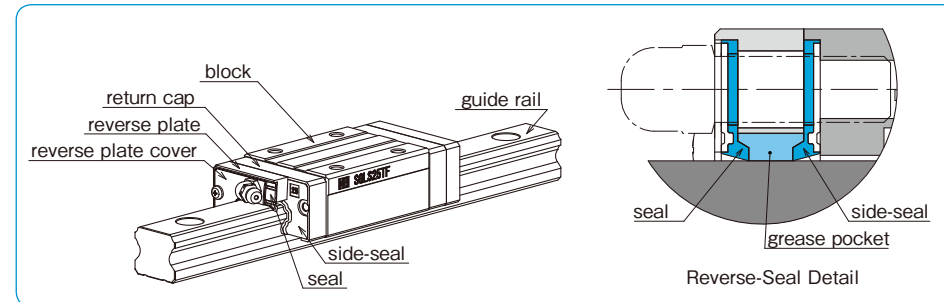
Figure A-32 Reverse-Seal
