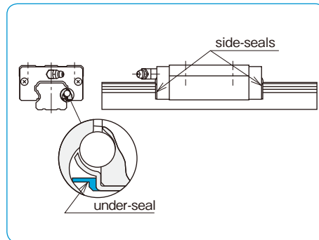
Figure A-24 Side-Seal and Under-Seal
