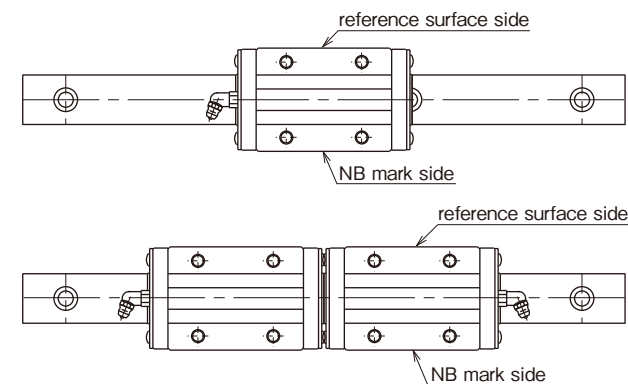
Figure A-59 Grease Fitting Orientation
