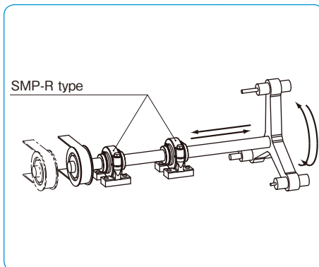
Application Example 3 Tool Changer
