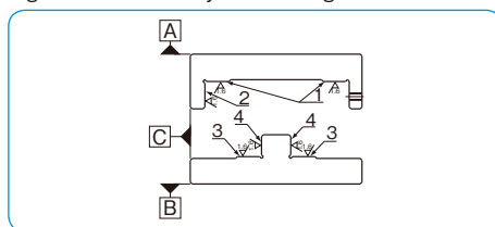
Figure G-12 Accuracy of Mounting Surface
