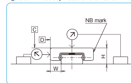
Figure G-21 Accuracy Measurement Method
