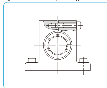
Figure C-7 Flange Type
