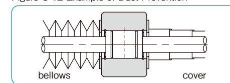
Figure C-12 Example of Dust Prevention
