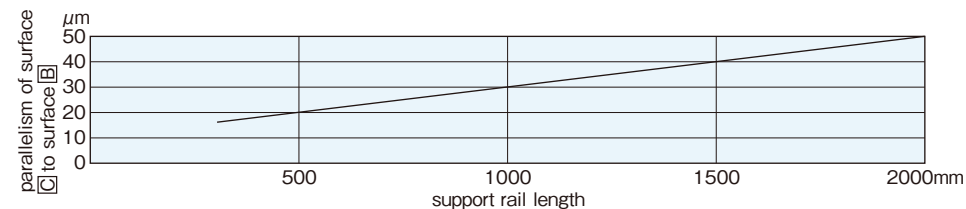
Figure C-18 Accuracy of CE/CD-type Support Rails
