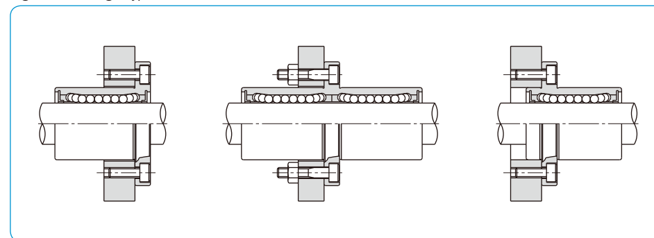
Figure C-7 Flange Type
