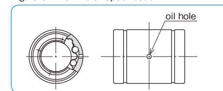
Figure C-11 Oil Hole - Specification-
