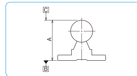
Figure C-17 Accuracy Measurement
