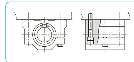
Figure C-20 Special Installation of SMJ Type
